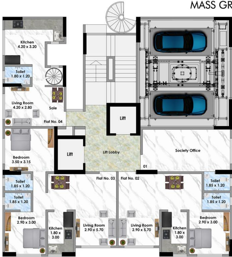
Third, Fifth and Eighth Floor Plan
