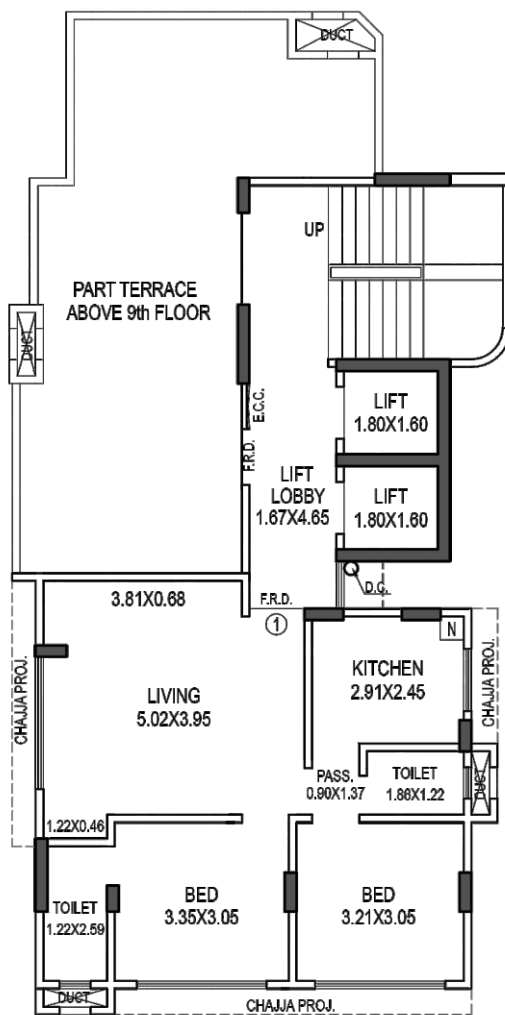
10th FLOOR PLAN
