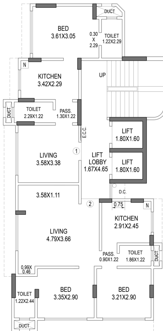
4th FLOOR PLAN
