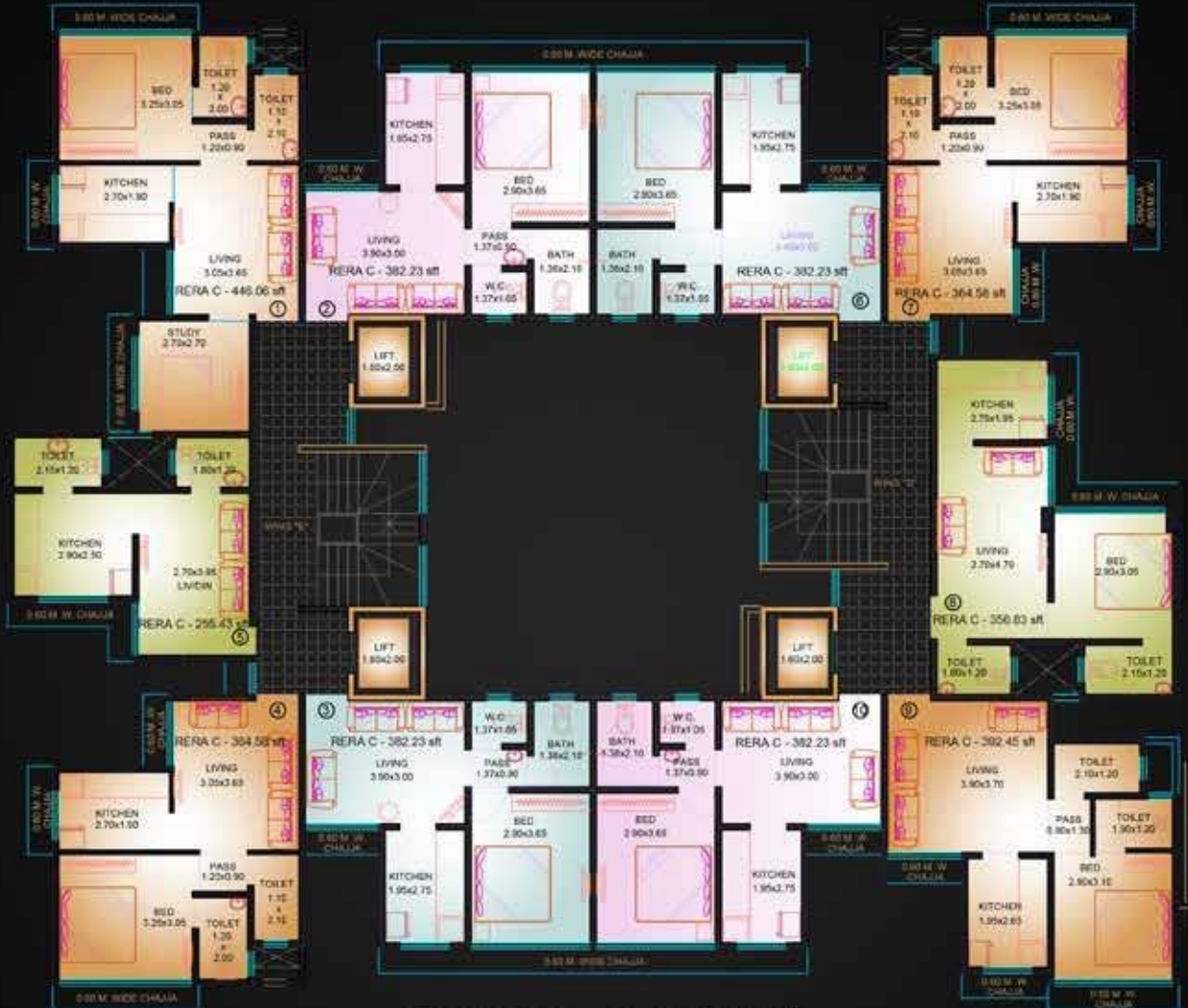
TYP FLOOR 1st to 7th (WING 'D' & 'E')
