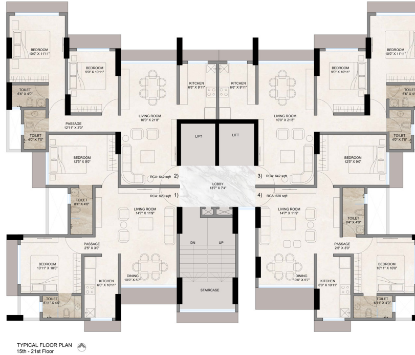
15 th - 21 st Typical Floor Plan
