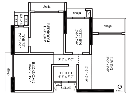
Layout for 622 SF RERA CARPET
