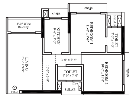
Layout for 639 SF RERA CARPET
