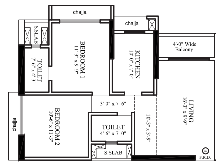
Layout for 659 SF RERA CARPET
