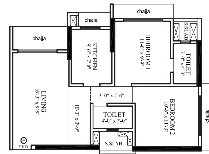
Layout for 602 SF RERA CARPET
