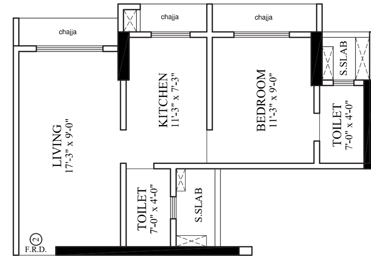
Layout for 412 SF RERA CARPET
