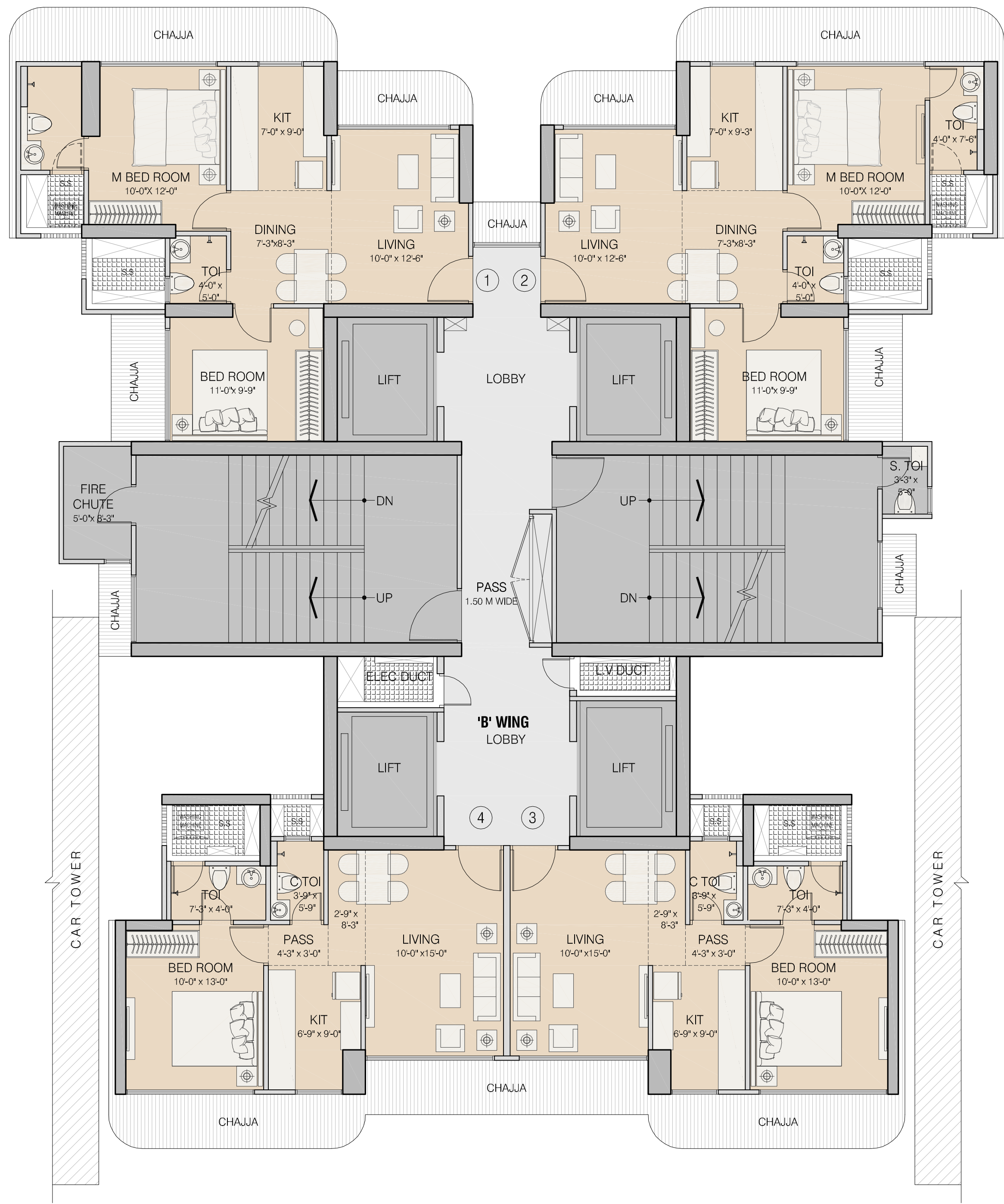
2nd TO 20th FLOOR PLAN
