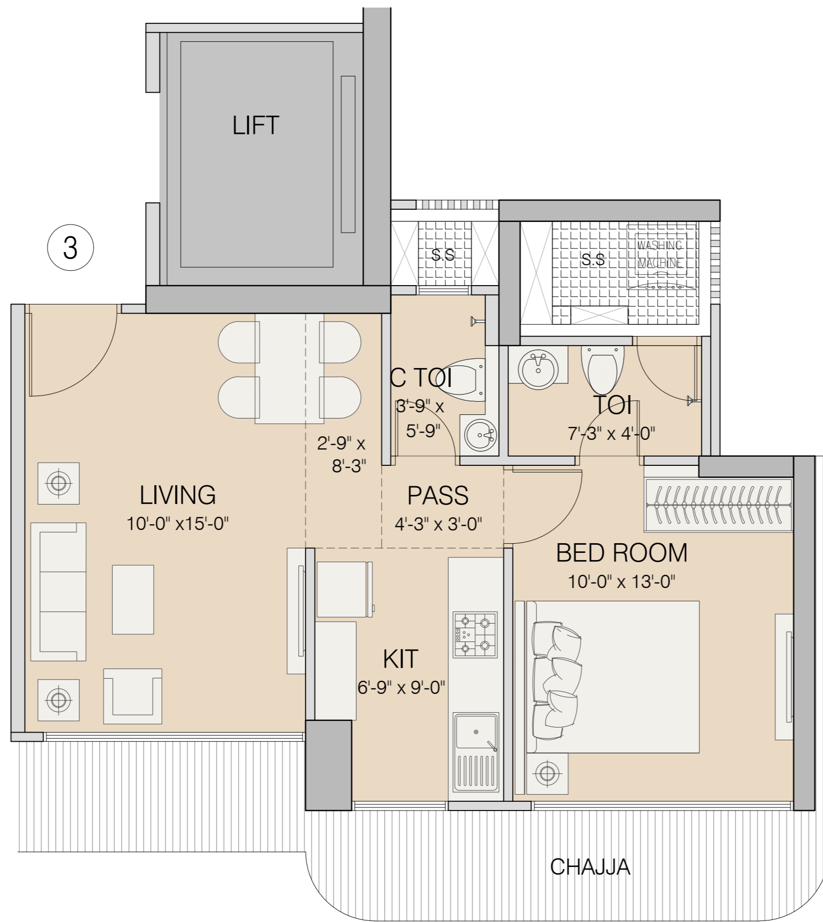
UNIT PLAN - 1BHK
