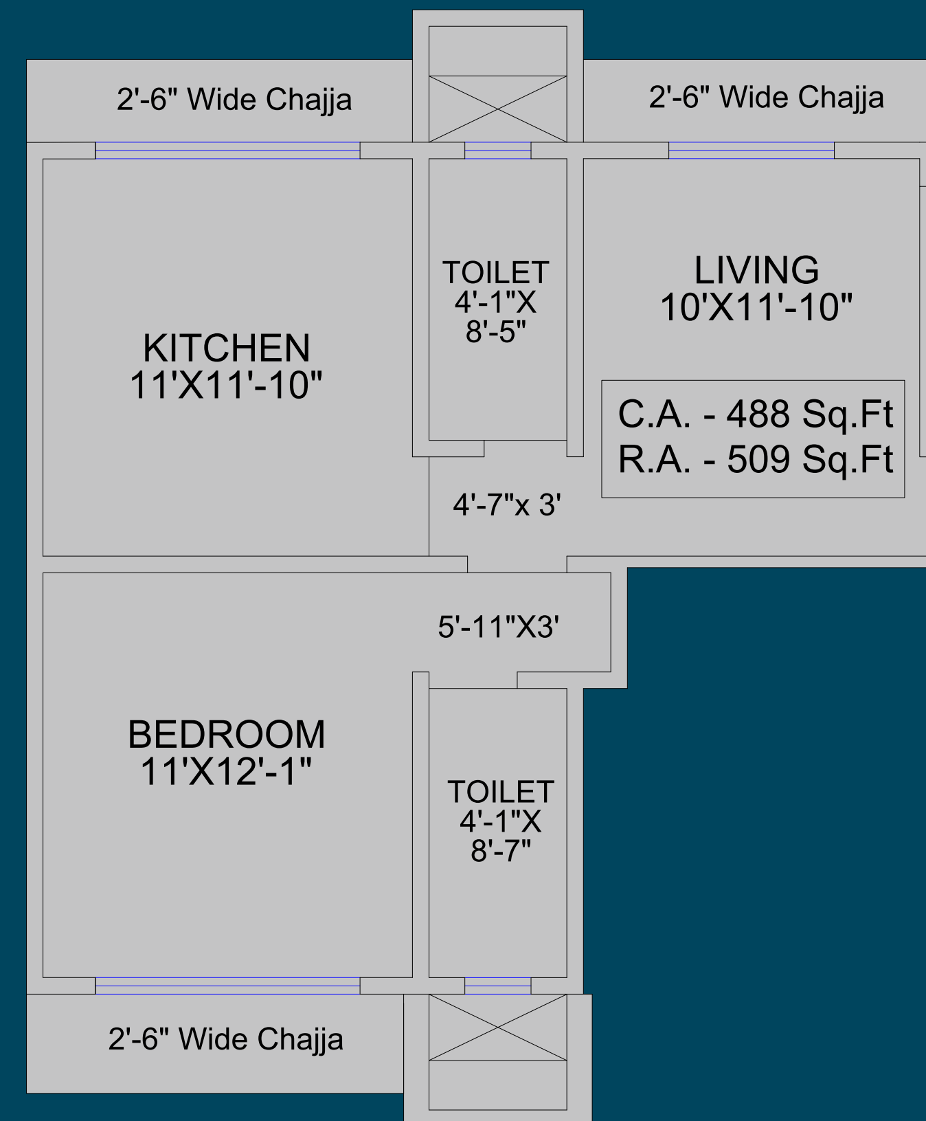
1 BHK – 509 Sqft Rera Carpet Area
