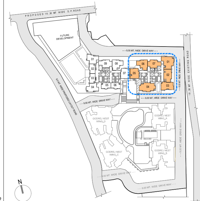
MASTER LAYOUT (KEY PLAN)
